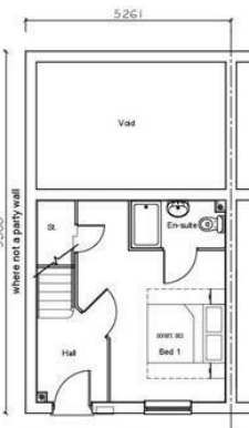
Ground Floor Plan (AS) Total Floor Area: 1182 sq' / 109.9 m²
